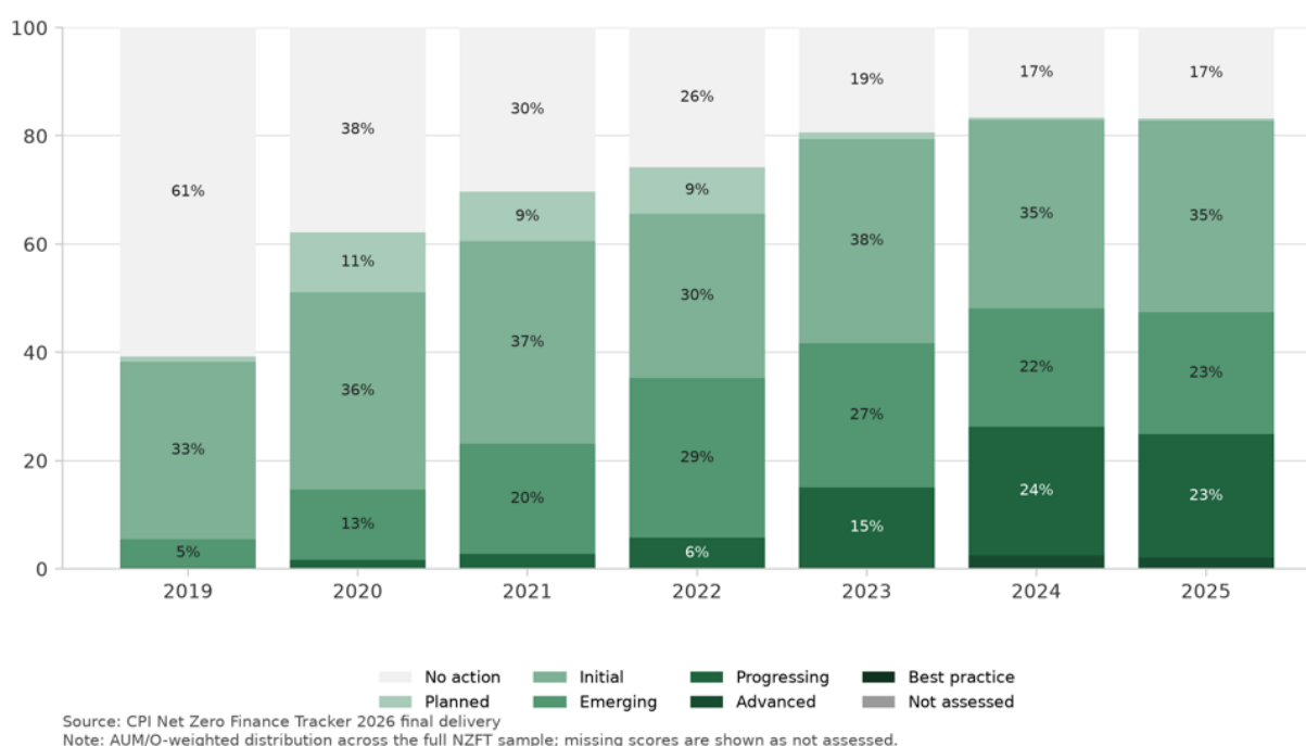
Figure 5: Example of score distribution by AUM/O
