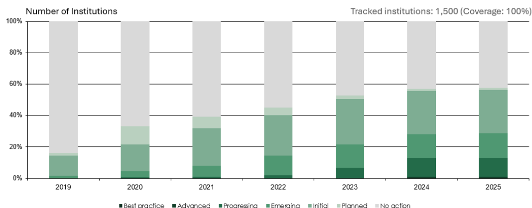
Figure 4: Example of score distribution by number of institutions
