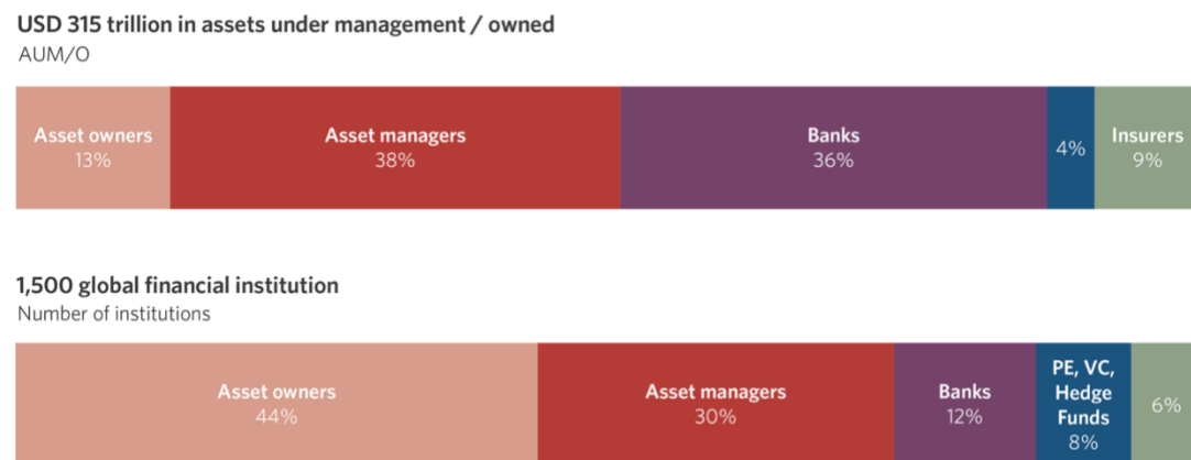
Figure 7: NZFT sample composition
